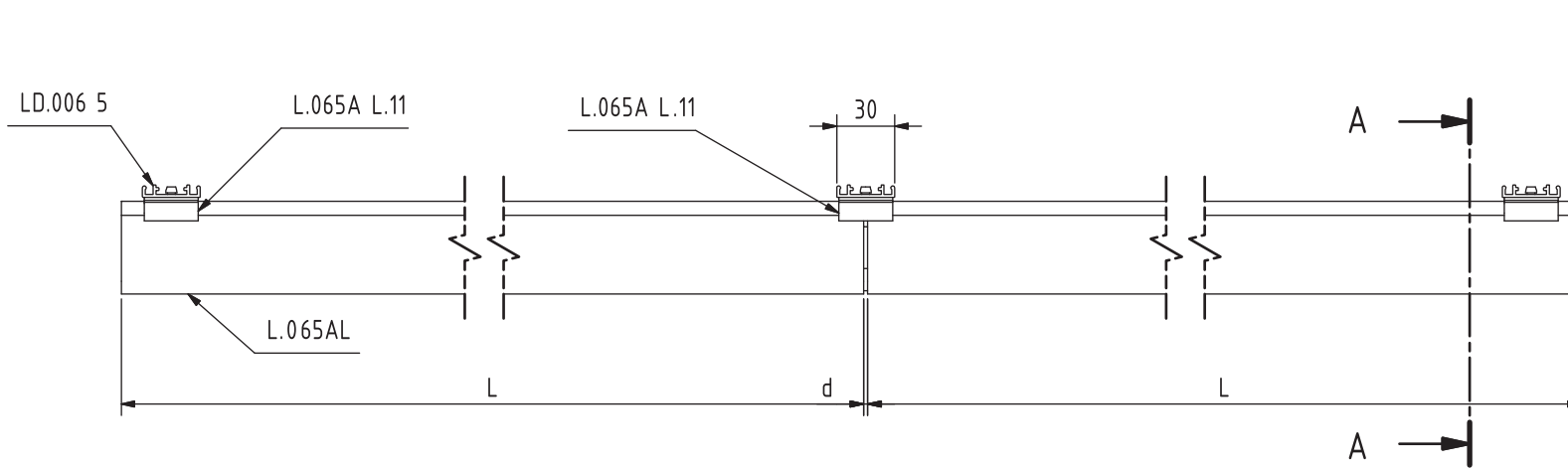
TOP VIEW
